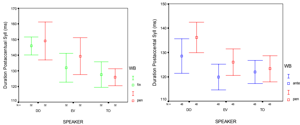
Figure 13. Mean values of duration of the postaccentual syllable (in ms) as a function of within-word position for all Spanish speakers: fin vs pen (graph on the left) and pen vs ante (graph on the right).
