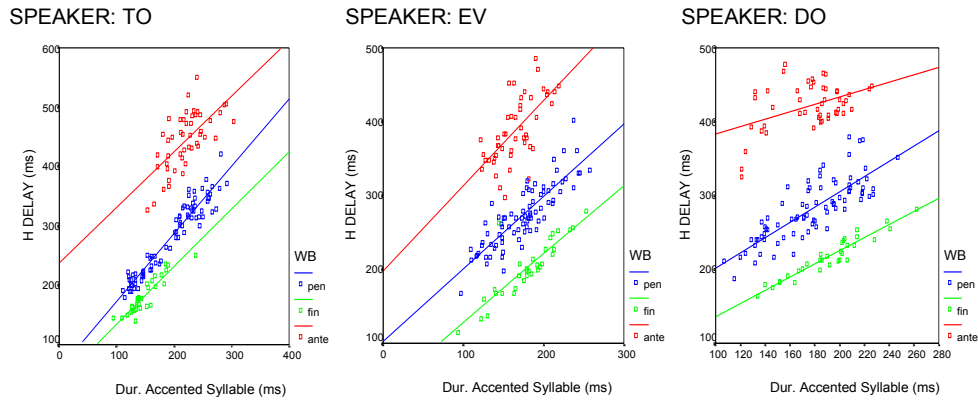
Figure 3. Peak delay as a function of the duration of the accented syllable in ms in three stress conditions (words with final, penultimate and antepenultimate stress) in Spanish for speakers TO, EV, and DO.
